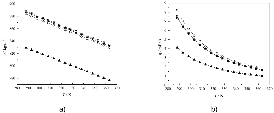
a) b) Fig. 2. a) Density and b) viscosity at atmospheric pressure of ( \square ) SME [2], ( \circ ) SEE [2], ( \star ) USME and ( \blacktriangle ) EuroDiesel [9].
